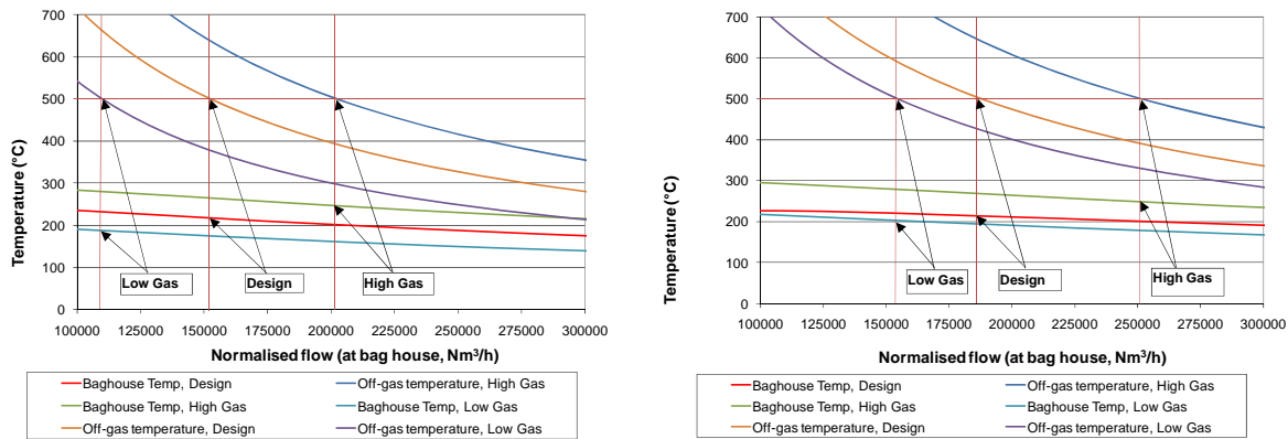
Figure 4: Off-gas profile along system for scenarios for furnaces 1-3 (left) and 4 (right)
