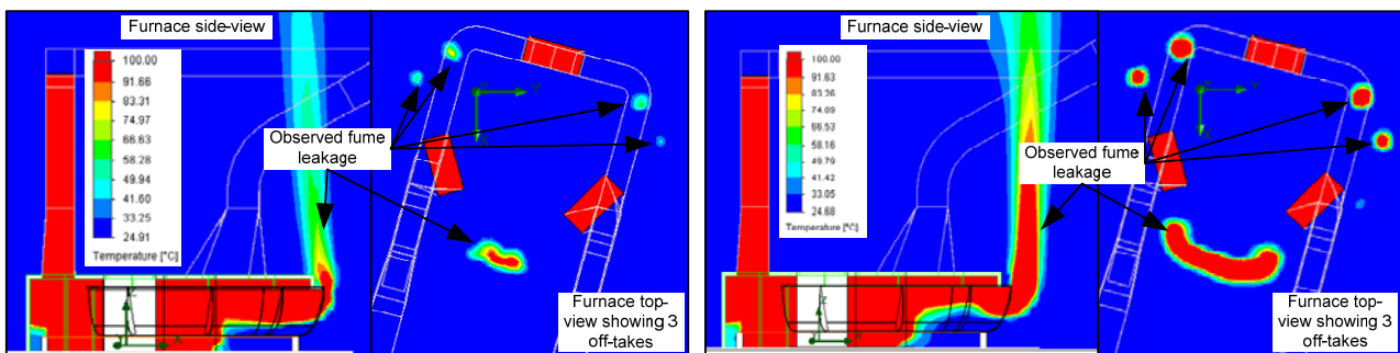
Figure 8: CFD results for 1 door open (left) and 3 doors open (right)
