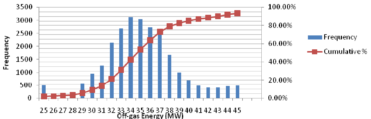
Figure 2 : Histogram indicating off-gas energy
