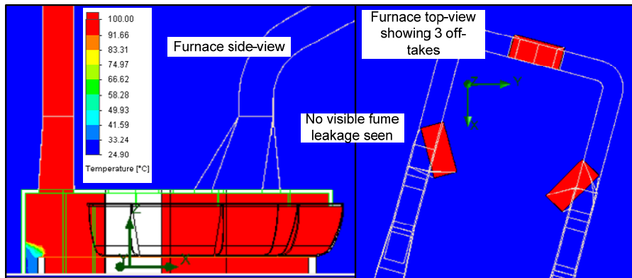
Figure 7: CFD results for 0 doors open
