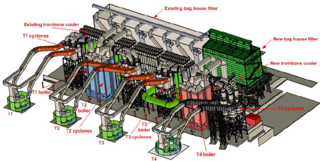
Figure 3: East Plant layout
