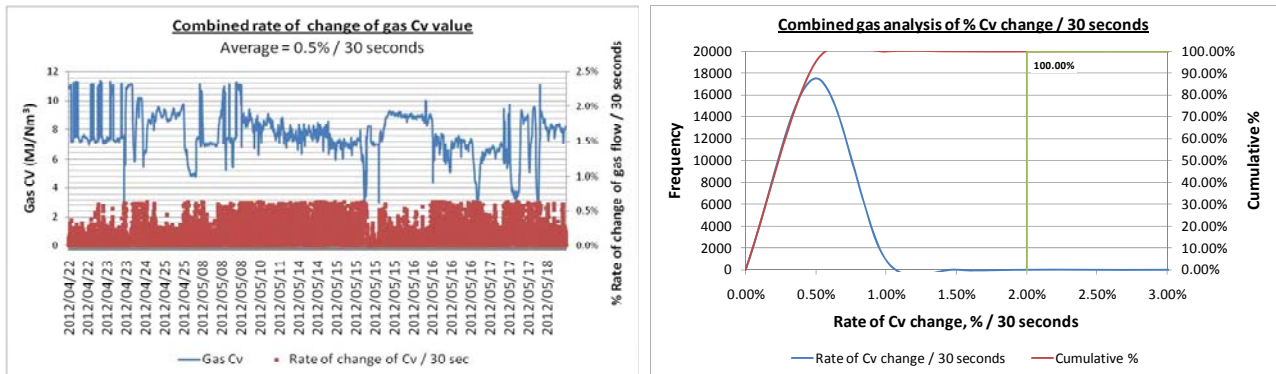
Figure 9: Calorific value assessment and Cv rate of change histogram and OGIVE curve
