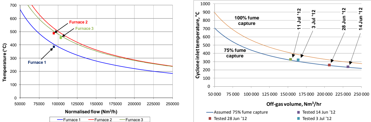
Figure 5: Off-gas design vs. tested conditions for furnaces 1-3 (left) and 4 (right)
