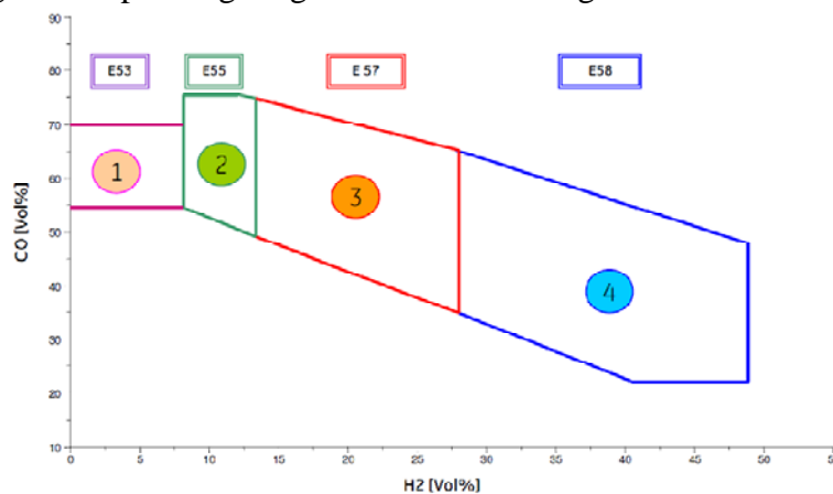
Figure 10: Engine selection chart
