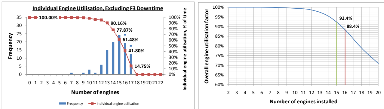
Figure 11: Individual engine utilization and overall engine utilization
