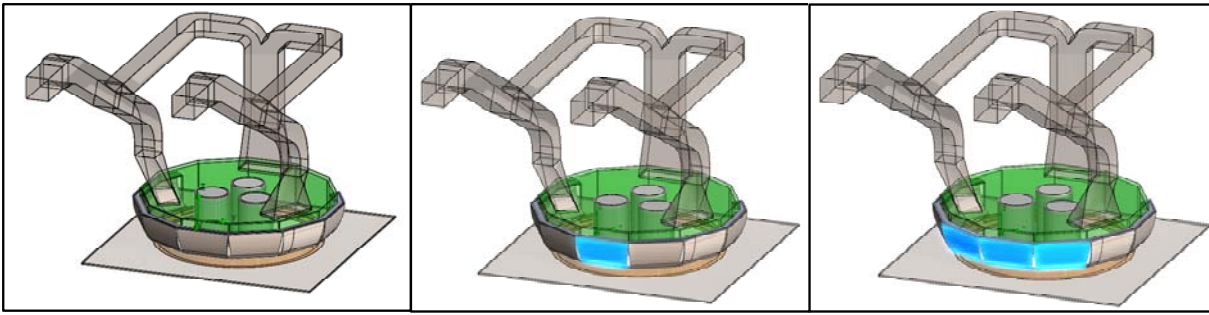
Figure 6: Furnace hood configurations for CFD scenarios
