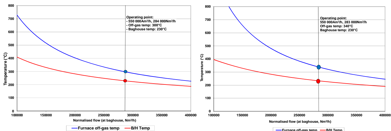
Figure 2: Off-gas model prediction with tapping fume fan on (Left) and off (right)
