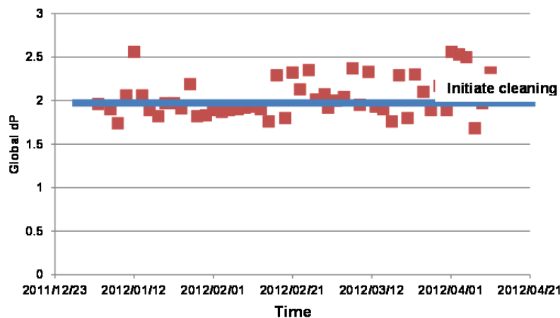
Figure 9: Global filter differential pressure
