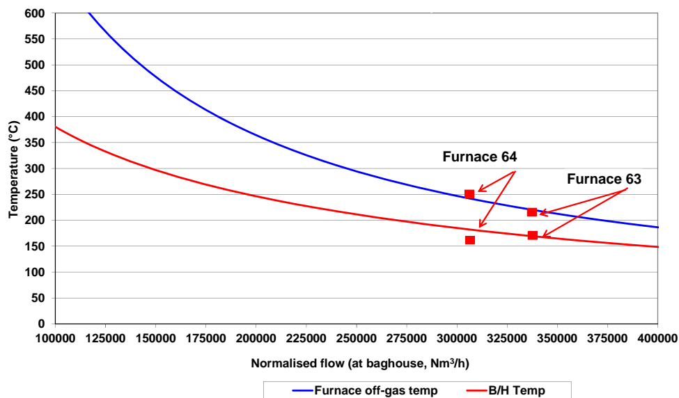
Figure 7: Off-gas design vs. tested conditions
