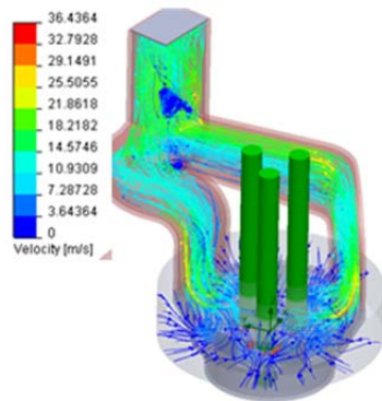
Figure 3: Elevation hood velocity
