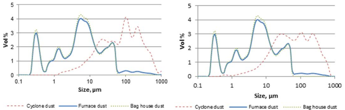
Figure 8: Furnace 63 (left) and furnace 64 (right) dust particle size distributions
