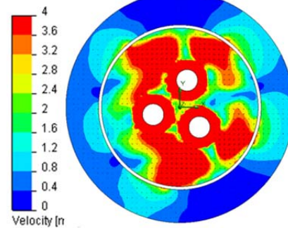
Figure 4 Hood plan view velocity
