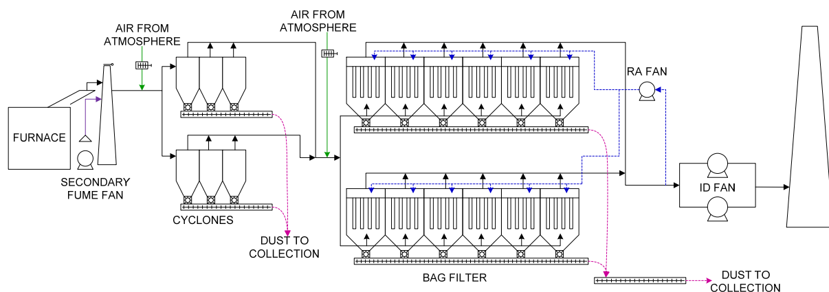
Figure 1: Basic off-gas system layout
