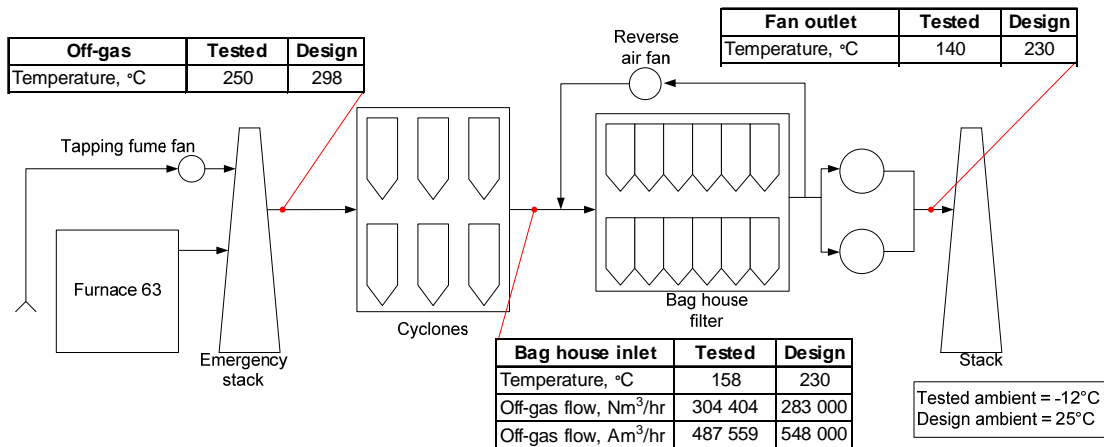
Figure 6: Flow testing results for Furnace 64
